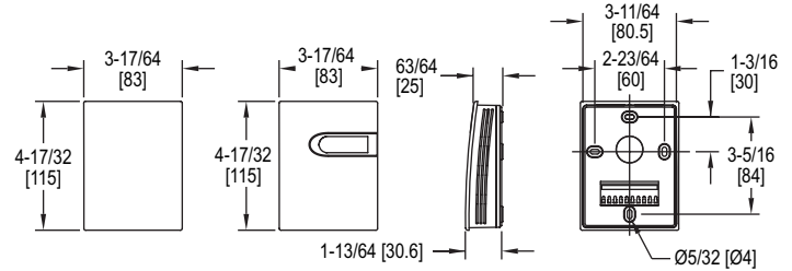
Wall mount
