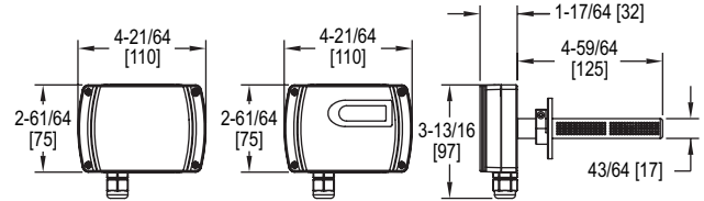
Duct mount
