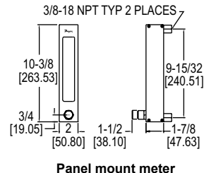
Panel mount meter
