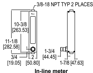
In-line meter
